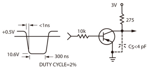
FIG.1 Delay and Rise Time Equivalent Test Circuit
