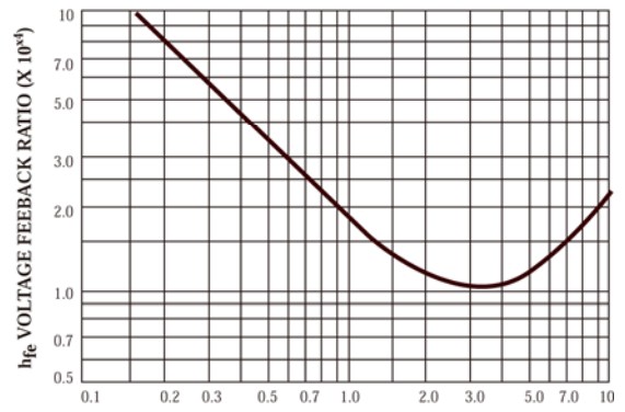
FIG.12 Votage Feedback Ratio
