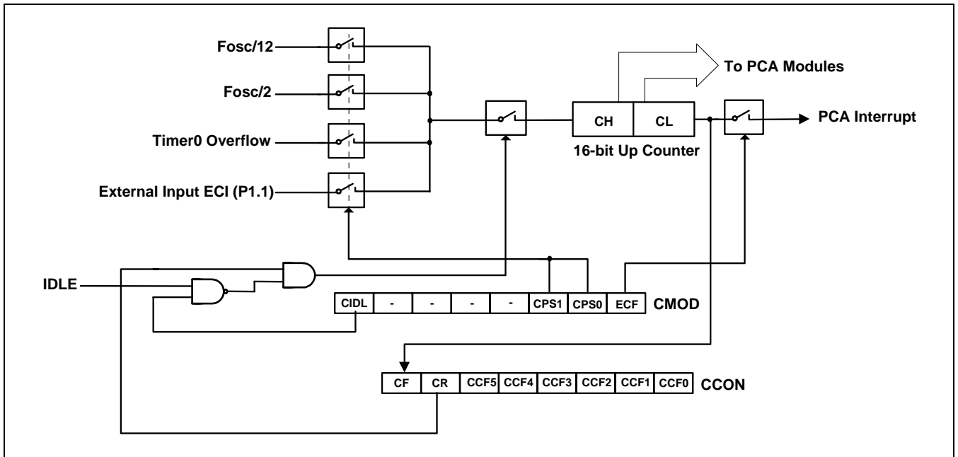
Figure 14-2. PCA Timer/Counter
